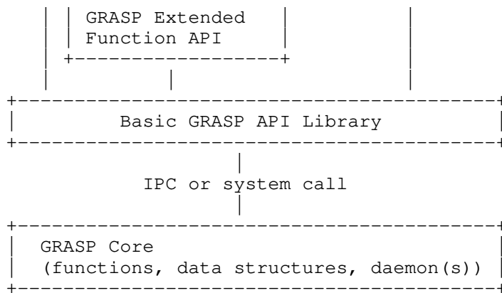
Figure 1: Software Layout
